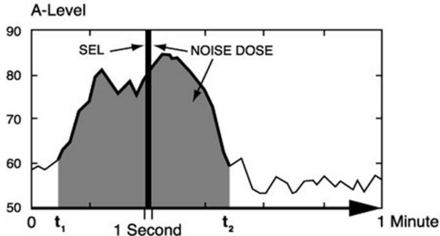
Figure E.1-2 Sound Exposure Level
