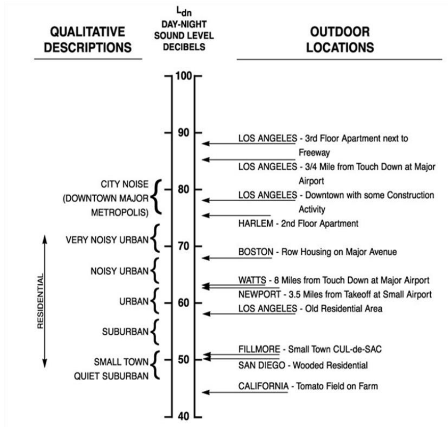
Figure E.1-4 Examples of Day-Night Average Sound Levels, DNL
