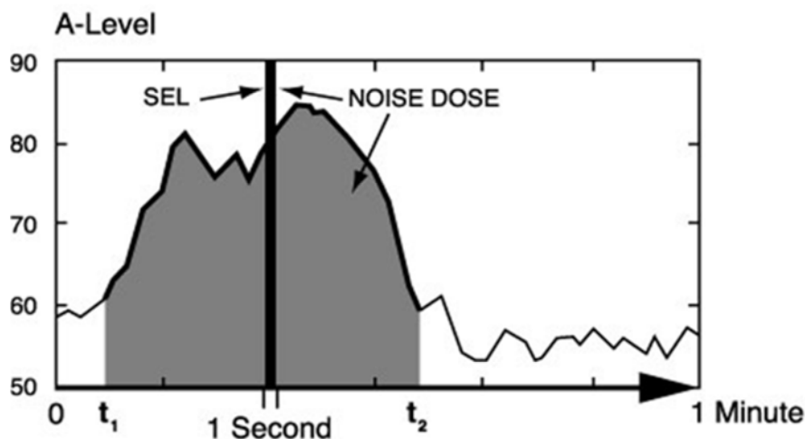
Exhibit E.1-2 Sound Exposure Level
