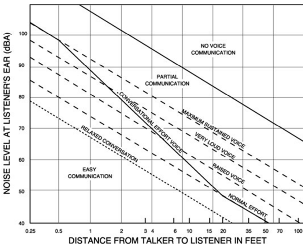
Exhibit E.1-5 Outdoor Speech Intelligibility
